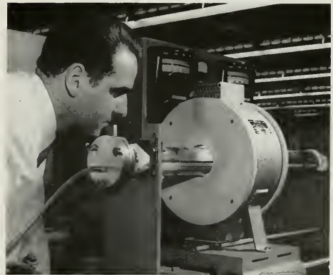
Germanium crystals are "grown" in high temperature electric furnace. Drum contains heating unit.
